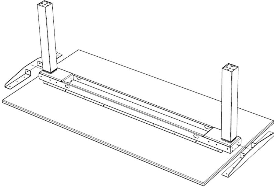
Figure 12 Positioning of the fixing plate (pos. B)
