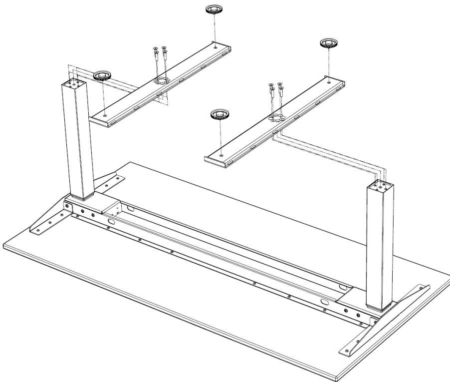
Figure 16 Screw connection of the foot base
