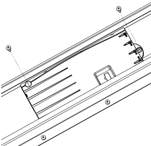
Figure 18 Installation of the controller
