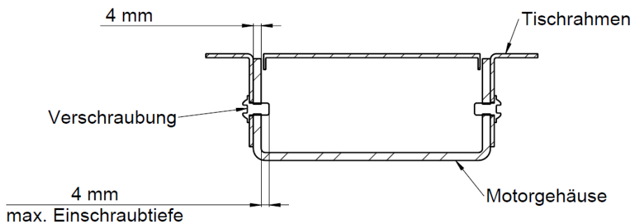
Figure 14 Maximum thread depth for the installation of the lifting columns
