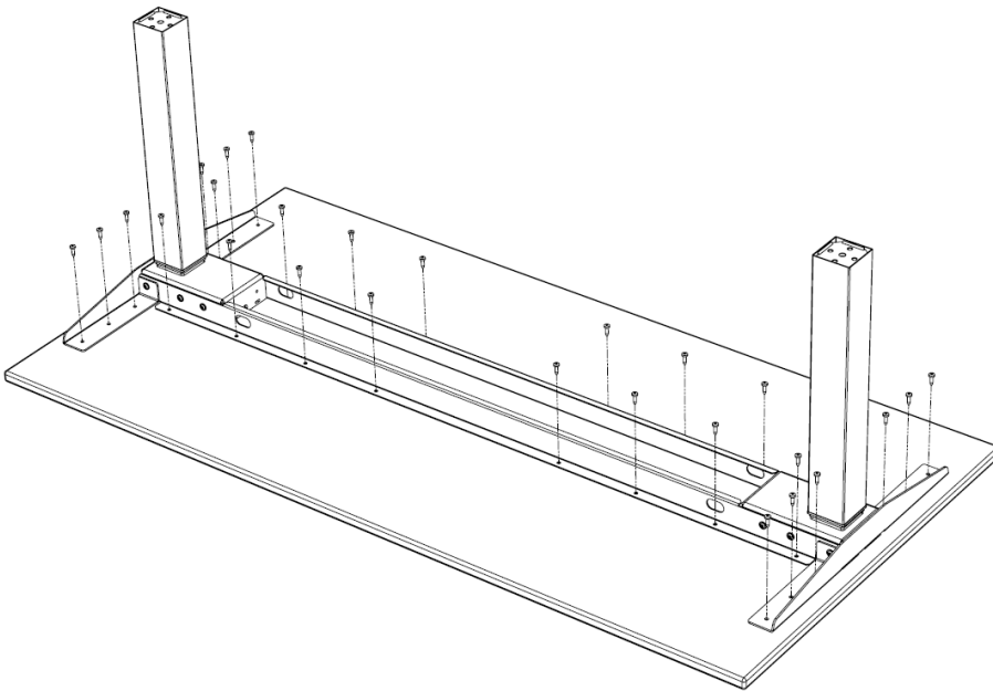
Figure 15 Screw connection of the table base frame
