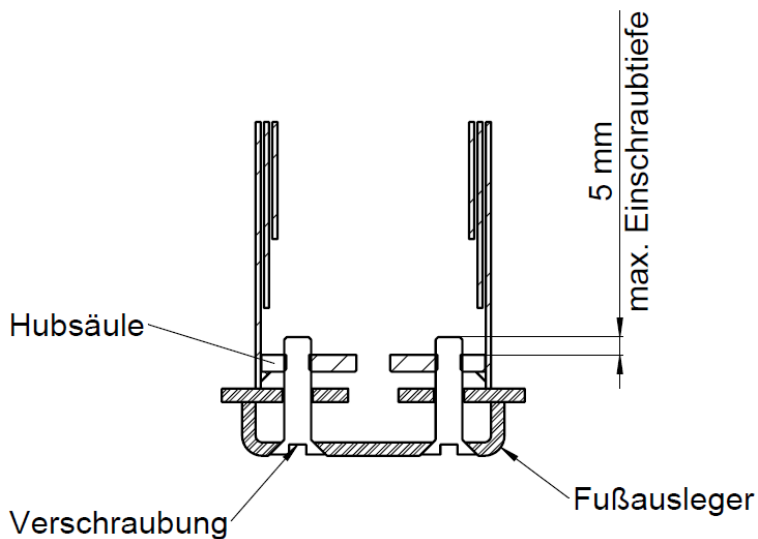
Figure 16 Screw connection of the foot base
