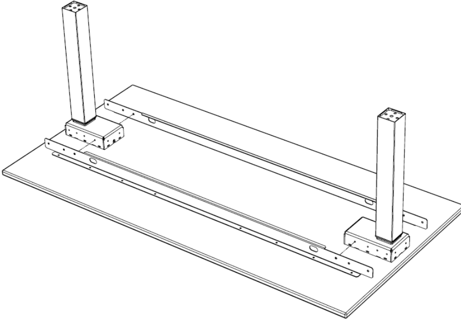
Figure 11 Positioning the cross beam (pos. A)
