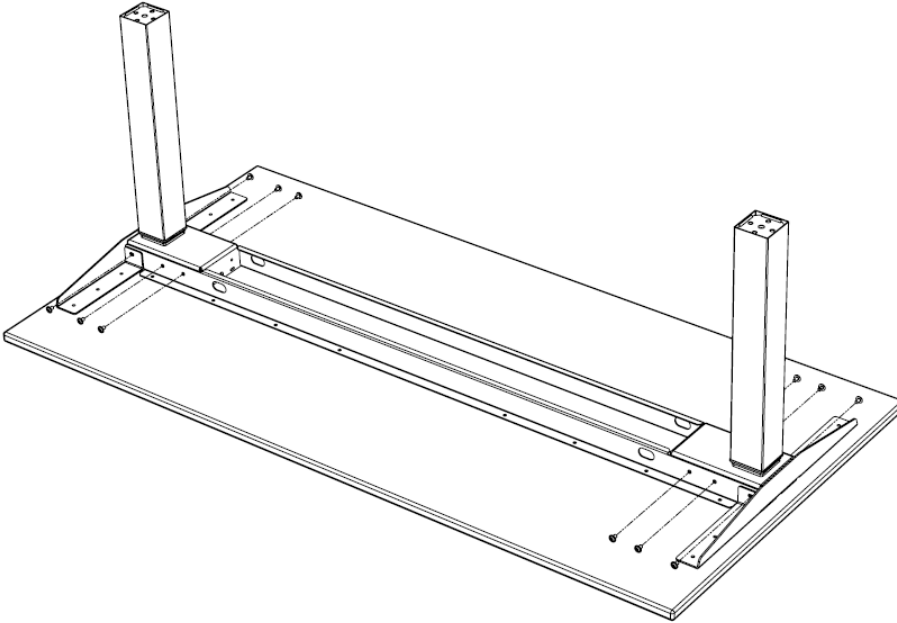
Figure 13 Cross beam screw connections
